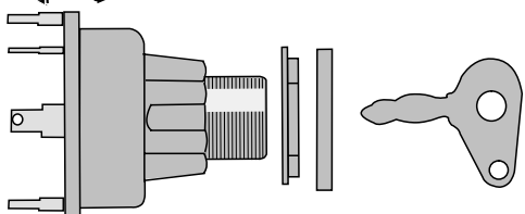
11. DECK / NET EMPTY SWITCH / SWEEPER LIFT PT/NO: 448001500
