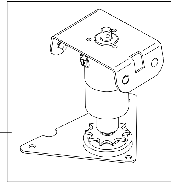
COMFORT STEERING ASSEMBLED VIEW
